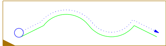
Toolpath left to the contour
